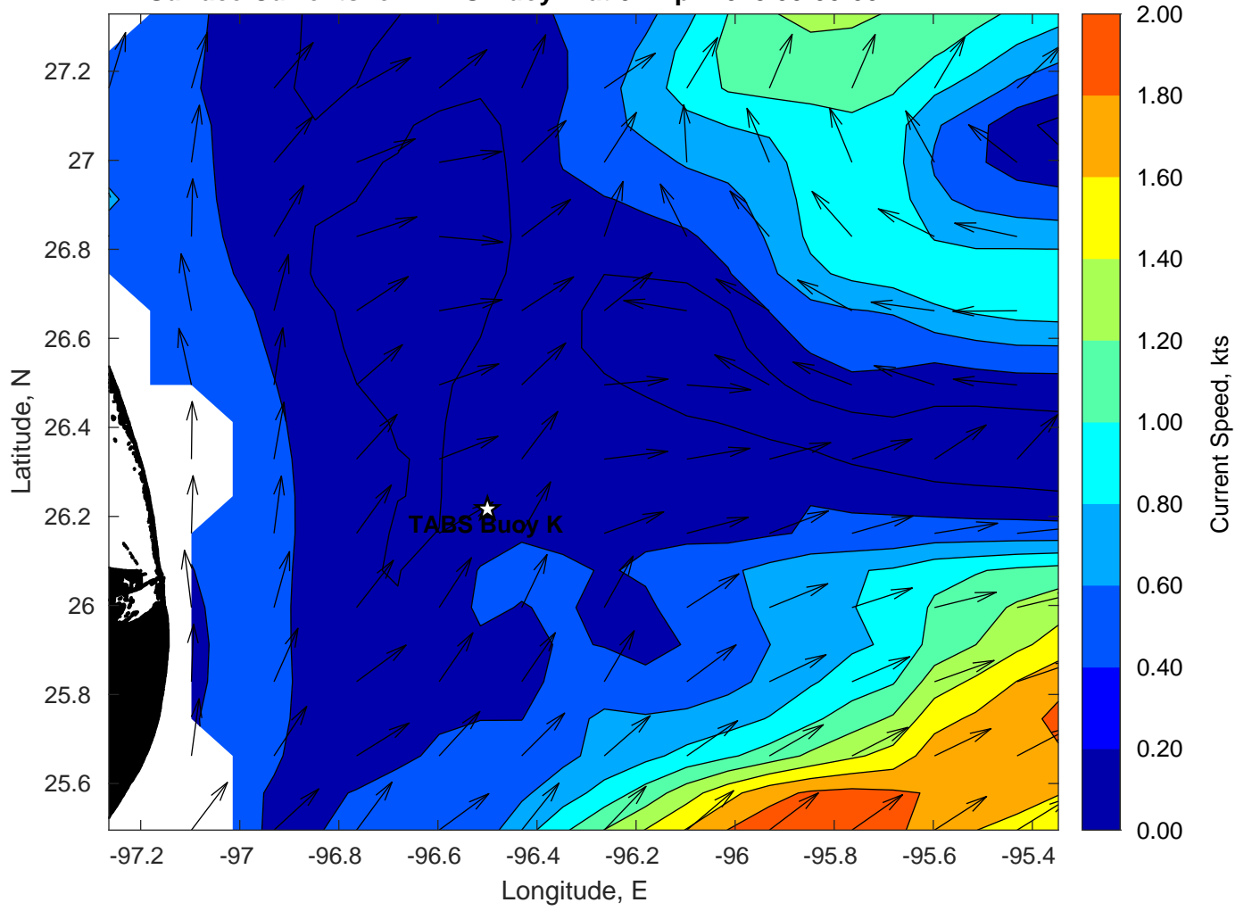
Surface Currents for TABS Buoy K at 04-Apr-2023 00:00:00
